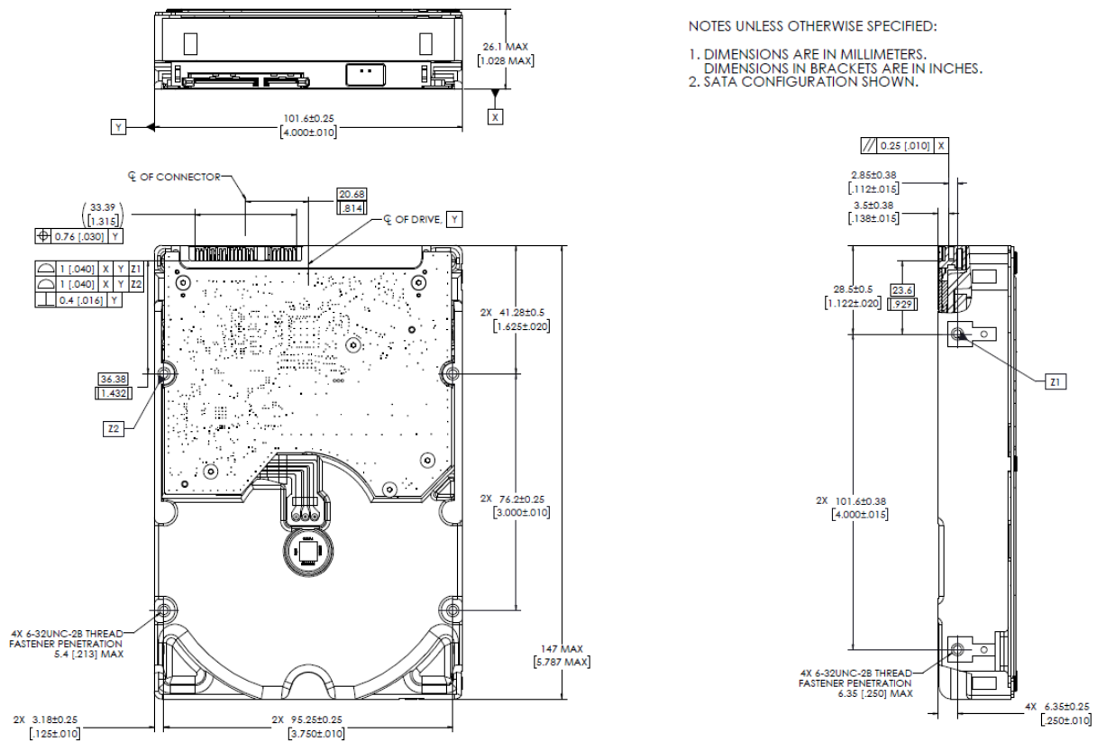
Figure 2-1. Mounting Dimensions
