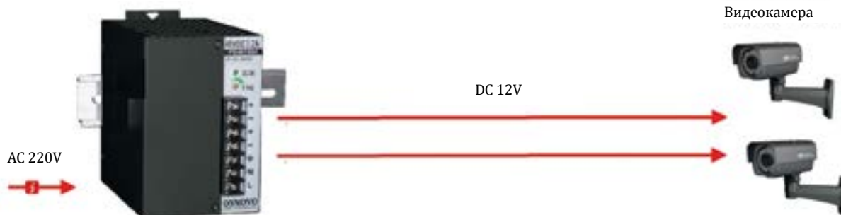
PS-12150/I
