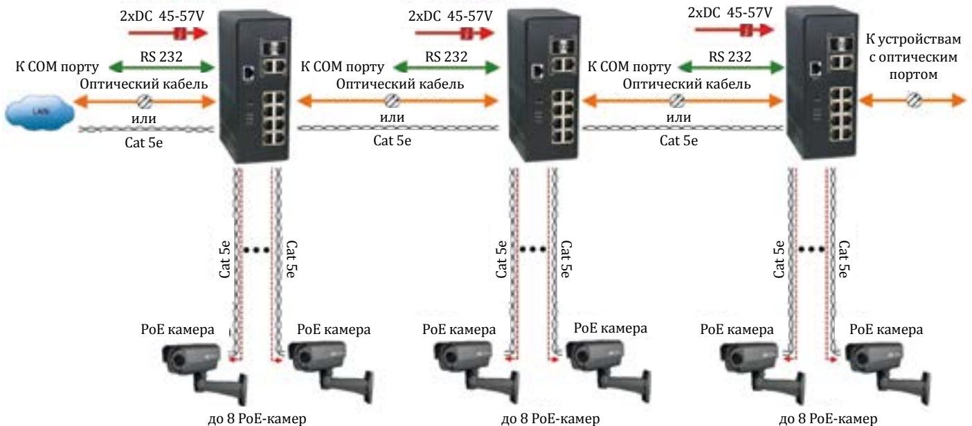
SW-80822/ILC
