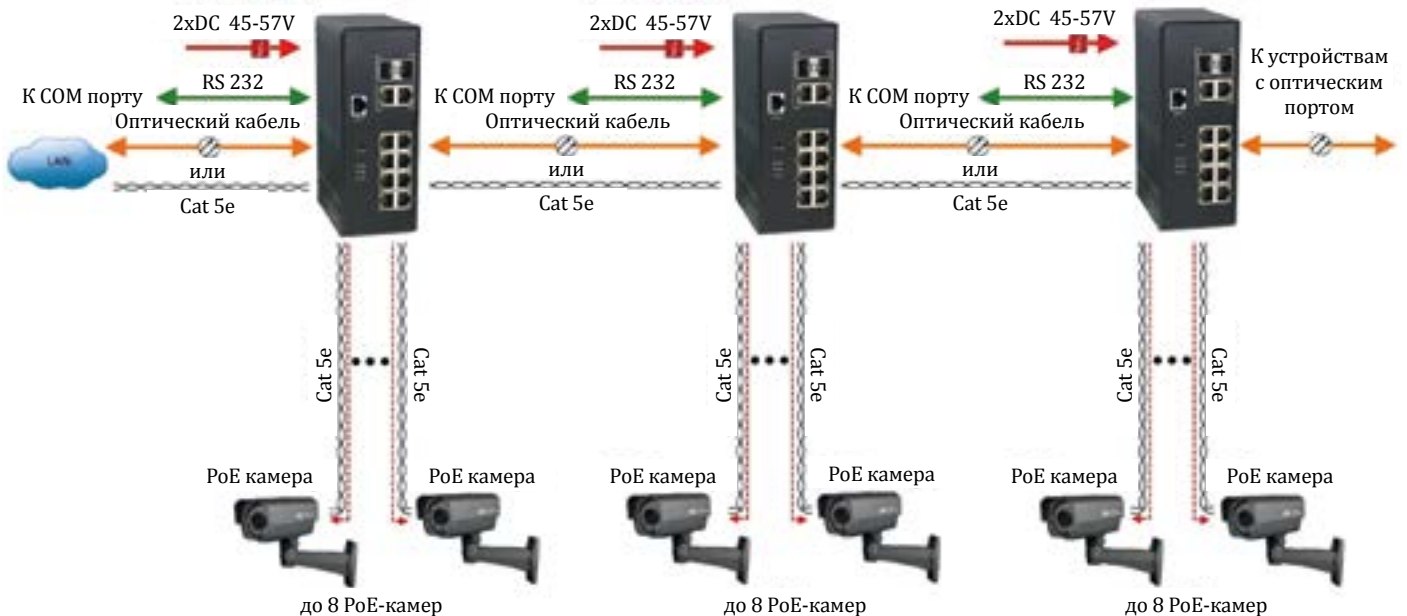
SW-60822/ILC
