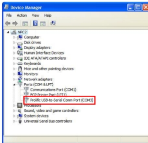
Figure 8 — Device Manager
